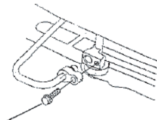
6 mm Bolt
